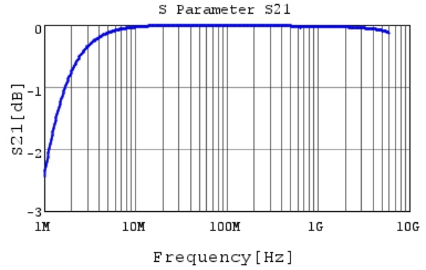
GRM1555C1H182JA01 S21 DCOV, 25degC
