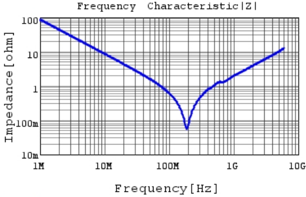
GRM1555C1H182JA01 |Z| DCOV, 25degC
