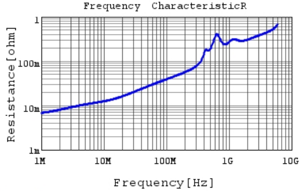
GRM1555C1H182JA01 R DCOV, 25degC
