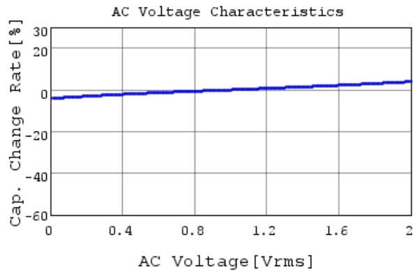
GCM31MR71H684KA55 C-AC Voltage capchange, Dc
