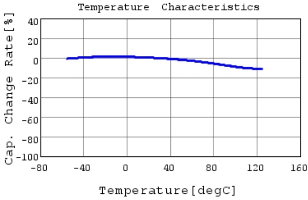
GCM31MR71H684KA55 C-Temp. capchange, DC0.0V,
