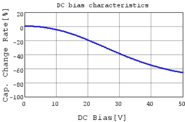
GCM31MR71H684KA55 C-DC bias capchange, 25.0c
