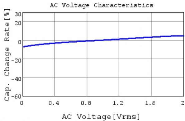
GRM188R61A474KA61 C-AC Voltage capchange, DC
