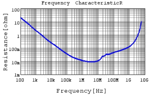
GRM188R61A474KA61 R DCOV, 25degC
