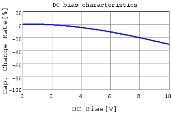
GRM188R61A474KA61 C-DC bias capchange, 25.0c
