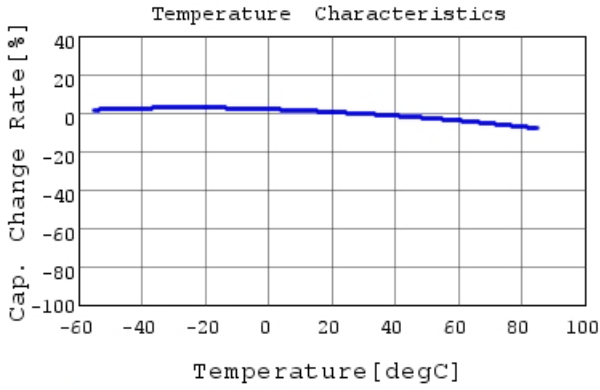
GRM188R61A474KA61 C-Temp. capchange, DC0.0V,
