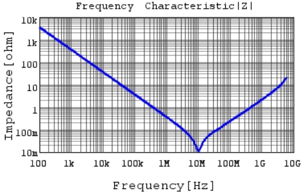
GRM188R61A474KA61 |Z| DCOV, 25degC
