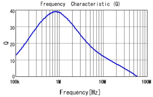
DFE252010P-1R2M Q
