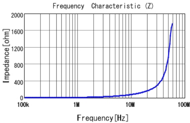
DFE252010P-1R2M |Z|
