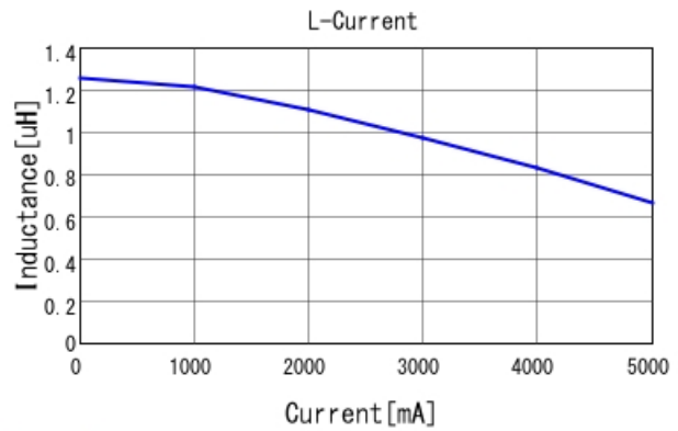
DFE252010P-1R2M L-Current 20degC
