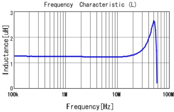
DFE252010P-1R2M L
