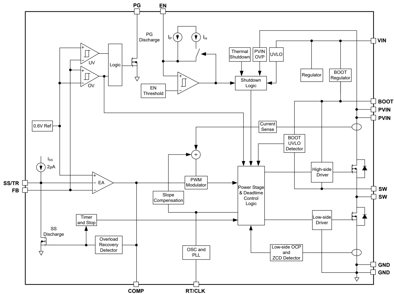
Figure 2. Block Diagram
