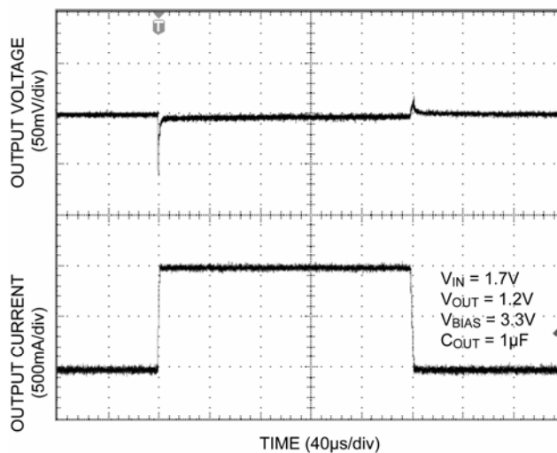
Load Transient
