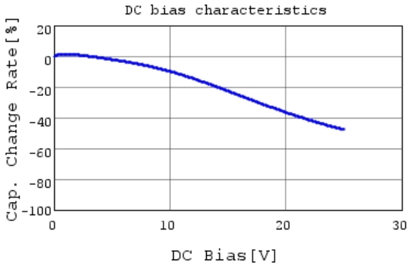
GRM155R71E223KA61 C-DC bias capchange, 25.0c
