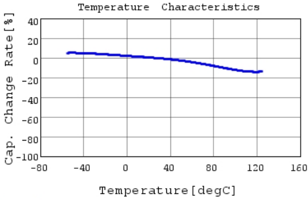
GRM155R71E223KA61 C-Temp. capchange, DC0.0V,
