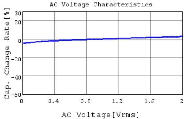
GRM155R71E223KA61 C-AC Voltage capchange, DC
