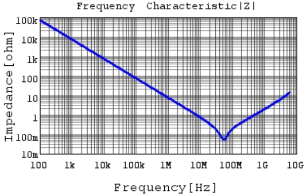
GRM155R71E223KA61 |Z| DCOV, 25degC
