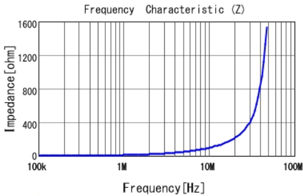
1239AS-H-1R5M |Z|
