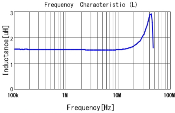
1239AS-H-1R5M L
