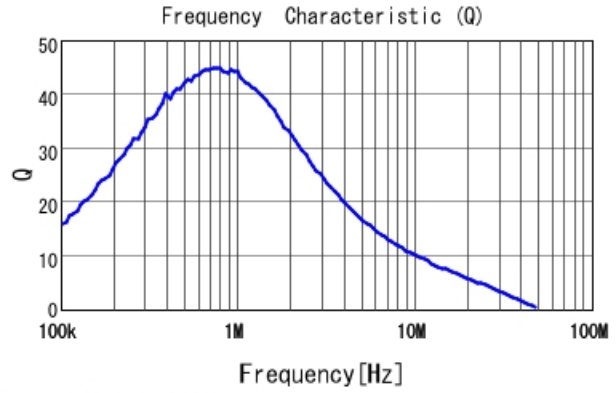
1239AS-H-1R5M Q
