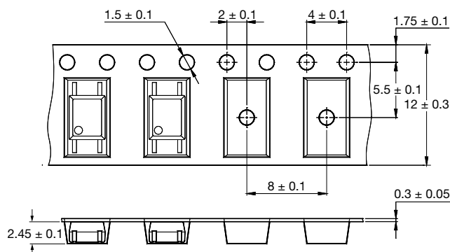
Fig. 18 - Tape Dimensions for 180° Rotation (T2)
