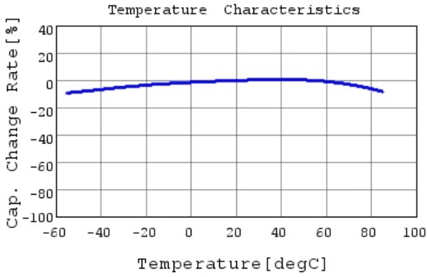
GRM21BR61H225KA73 C-Temp. capchange, DC0.0V,
