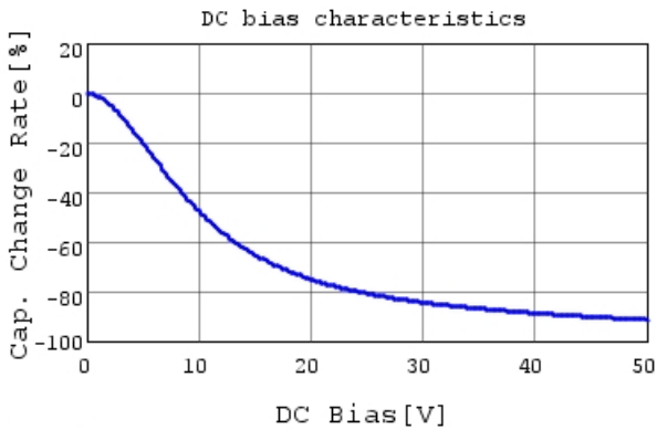
GRM21BR61H225KA73 C-DC bias capchange, 25.0c
