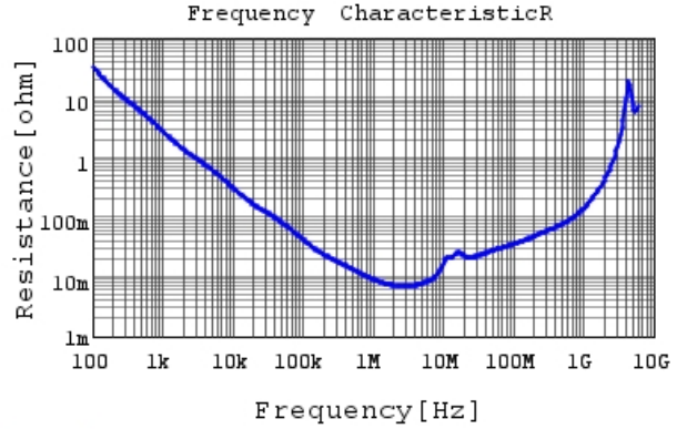
GRM21BR61H225KA73 R DCOV, 25degC
