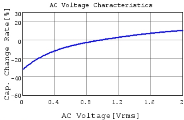
GRM21BR61H225KA73 C-AC Voltage capchange, Dc
