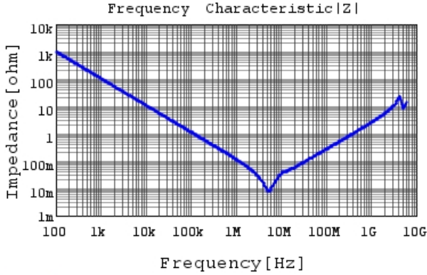
GRM21BR61H225KA73 |Z| DCOV, 25degC
