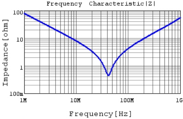
DE2E3KY222MN2AM01F |Z| DCOV, 20degC
