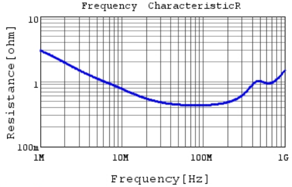
DE2E3KY222MN2AM01F R DCOV, 20degC
