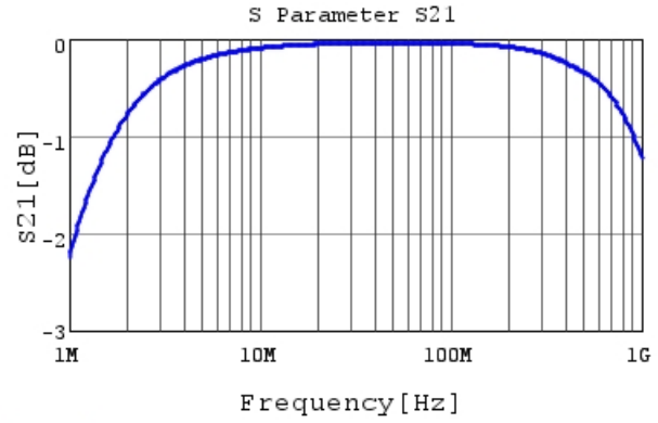
DE2E3KY222MN2AM01F S21 DCOV, 20degC
