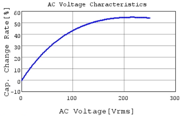
DE2E3KY222MN2AM01F C-AC Voltage capchange, I
