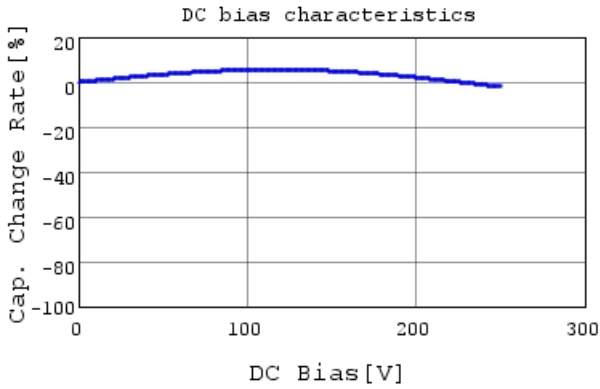
DE2E3KY222MN2AM01F C-DC bias capchange, 20.0
