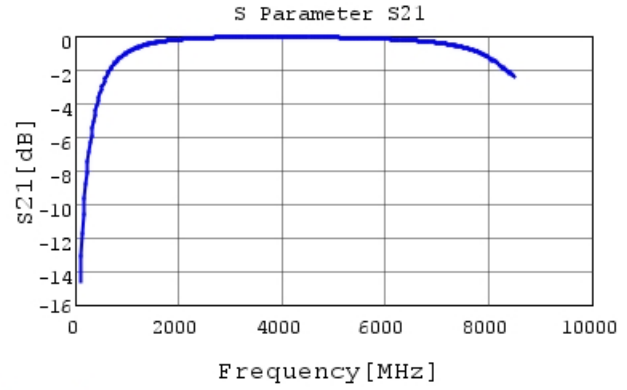
GRM1885C1H3R0CA01 S21 DCOV, 25degC
