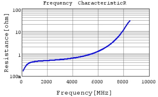
GRM1885C1H3R0CA01 R DCOV, 25degC
