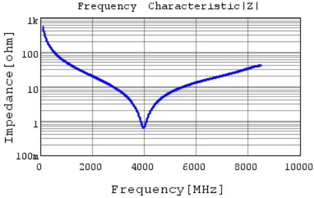
GRM1885C1H3R0CA01 |Z| DCOV, 25degC
