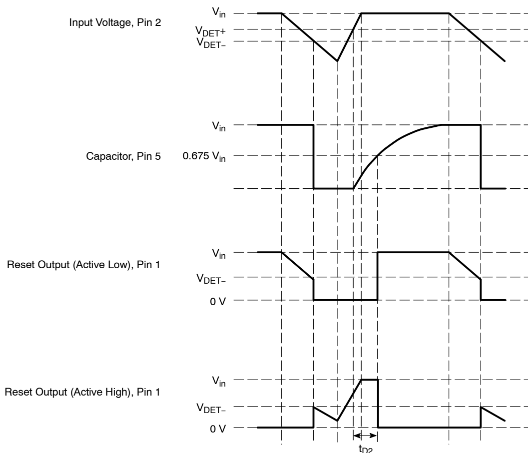
Figure 37. Timing Waveforms
