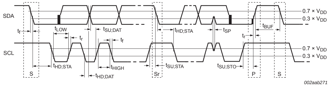
Fig 20. Timing diagram
