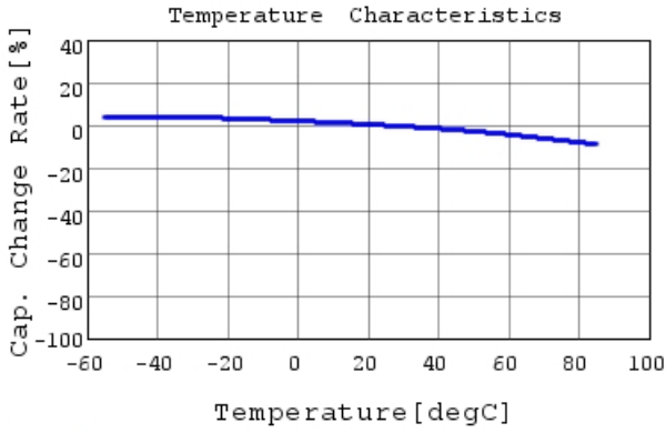
GRM219R61A105KA01 C-Temp. capchange, DC0.0V,
