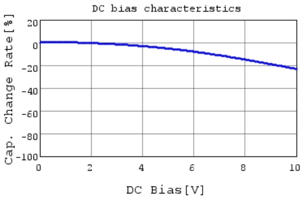
GRM219R61A105KA01 C-DC bias capchange, 25.0c
