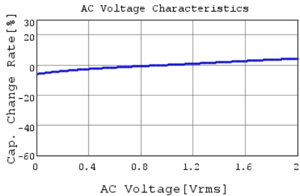
GRM219R61A105KA01 C-AC Voltage capchange, DC
