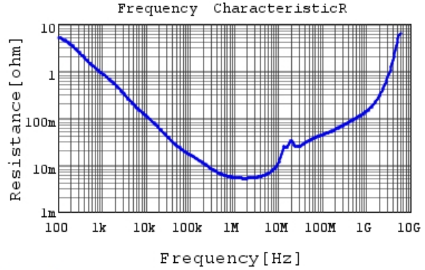
GRM219R61A105KA01 R DCOV, 25degC
