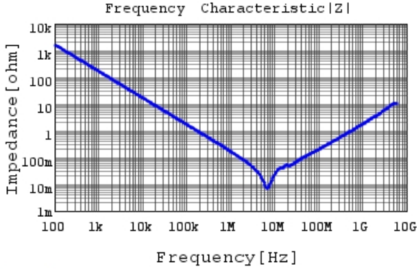
GRM219R61A105KA01 |Z| DCOV, 25degC
