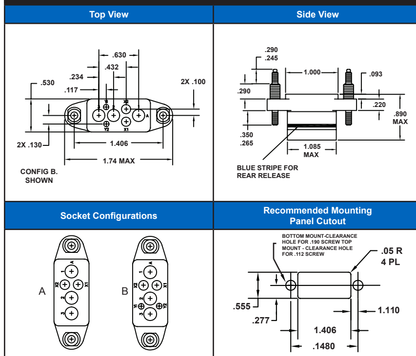
Relay Socket Dimensions
