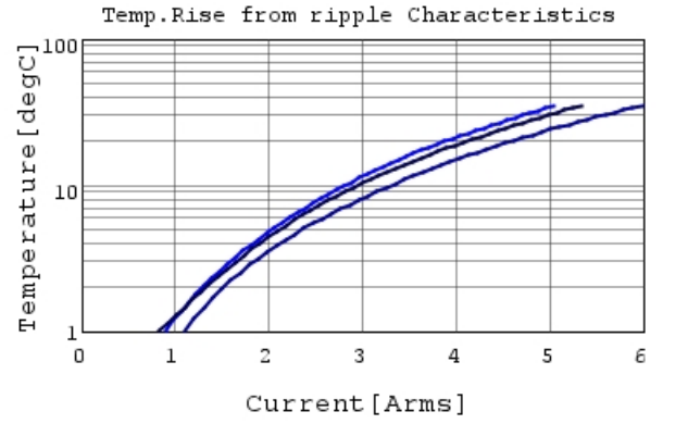
GRM31CR71A106KA01 Temp.rise — 100kHz —
