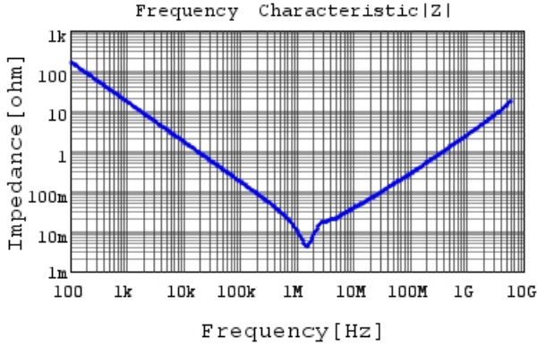
GRM31CR71A106KA01 |Z| DCOV, 25degC
