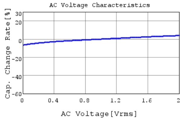
GRM31CR71A106KA01 C-AC Voltage capchange, Dc
