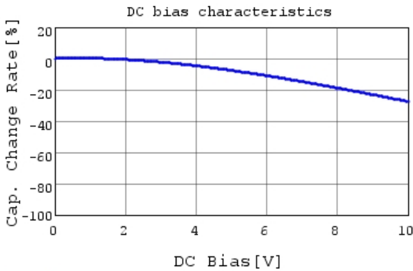
GRM31CR71A106KA01 C-DC bias capchange, 25.0c
