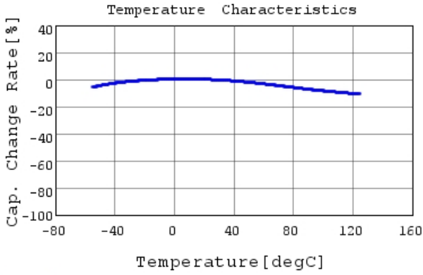
GRM31CR71A106KA01 C-Temp. capchange, DC0.0V,
