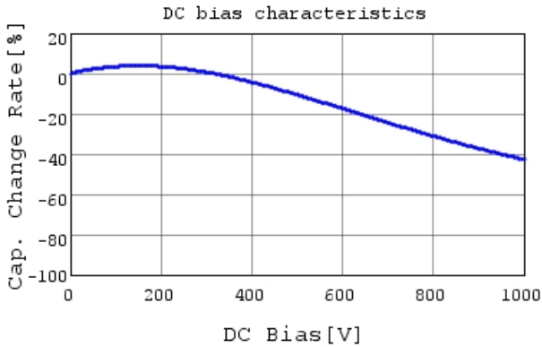
DE6E3KJ472MN3A C-DC bias capchange, 20.0degC
