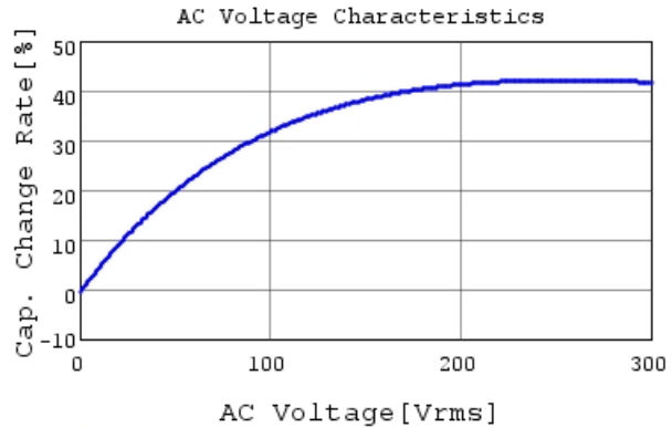
DE6E3KJ472MN3A C-AC Voltage capchange, DCOV,
