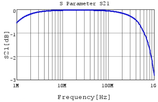
DE6E3KJ472MN3A S21 DCOV, 20degC
