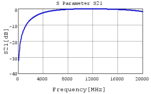
GRM1555C1HR40WA01 S21 DCOV, 25degC
