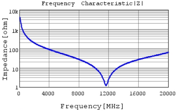
GRM1555C1HR40WA01 |Z| DCOV, 25degC
