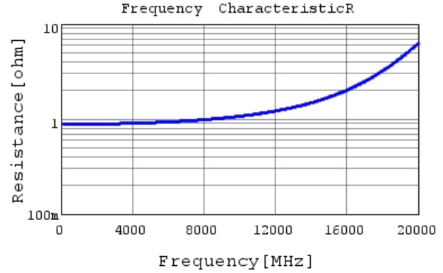
GRM1555C1HR40WA01 R DCOV, 25degC
