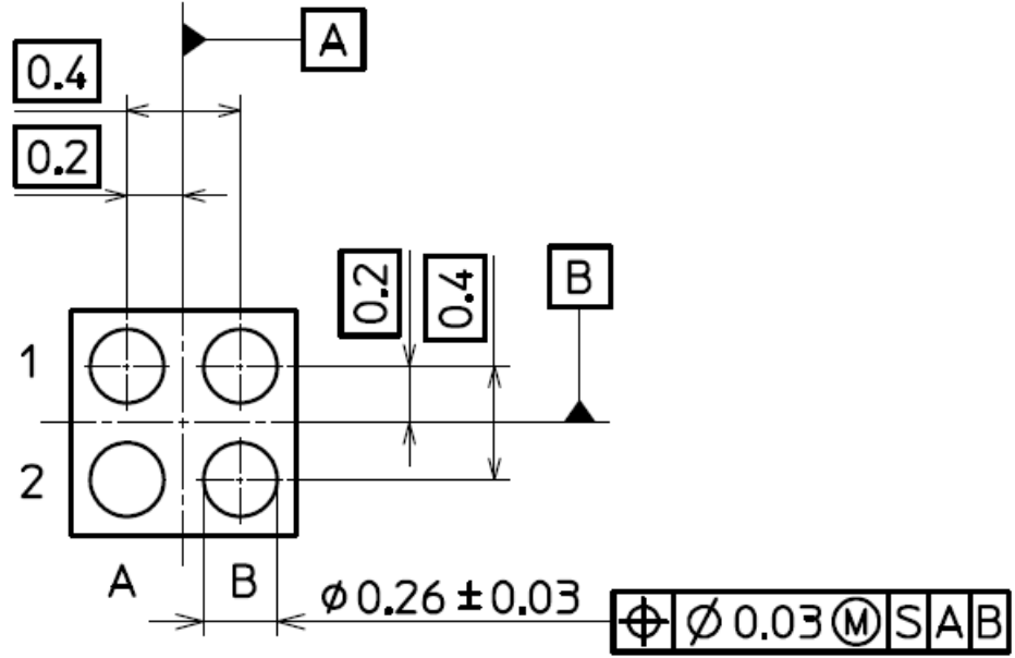
BOTTOM VIEW
