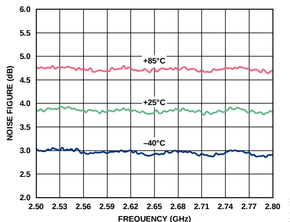
Figure 26. AMP2-2630 MHz: Noise Figure vs. Frequency and Temperature
