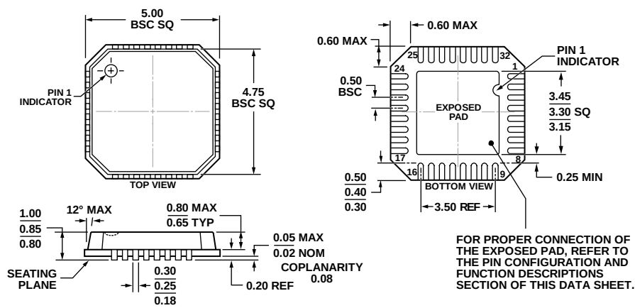
Figure 80. 32-Lead Lead Frame Chip Scale Package [LFCSP_VQ] 5 mm x 5 mm Body, Very Thin Quad (CP-32-3) Dimensions shown in millimeters
