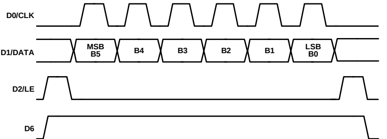
Figure 60. SPI Timing Sequence
