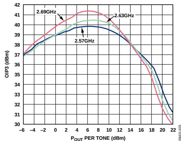
Figure 25. AMP2-2630 MHz: OIP3 vs. P_{OUT} and Frequency
