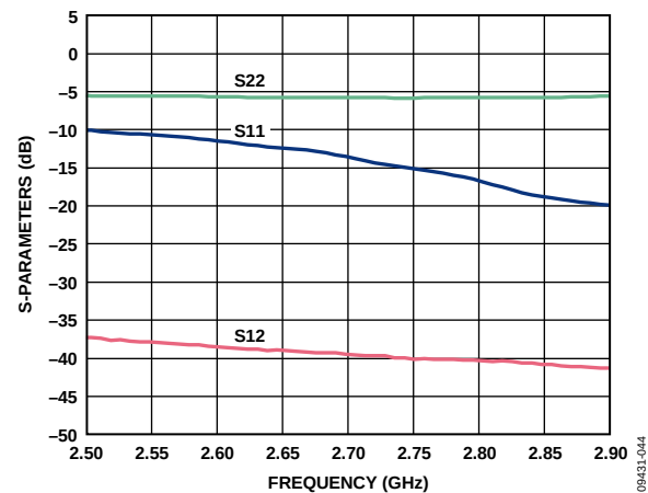
Figure 44. Loop-2630 MHz: Input Return Loss ( S_{11} ), Output Return Loss ( S_{22} ), and Reverse Isolation ( S_{12} ) vs. Frequency, Minimum Attenuation State
