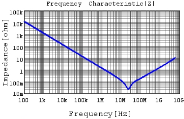
GRT155C81E224KE01 |Z| DCOV,25degC
