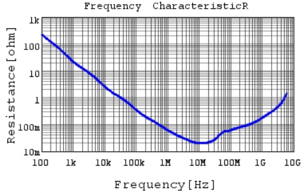
GRT155C81E224KE01 R DCOV,25degC
