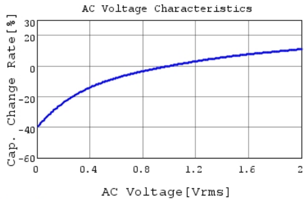
GRT155C81E224KE01 C-AC Voltage capchange, Dc
