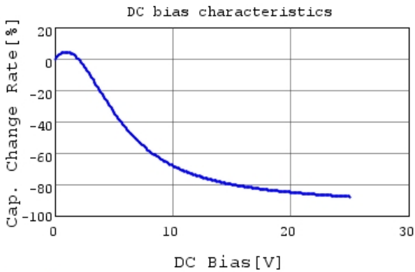
GRT155C81E224KE01 C-DC bias capchange, 25.0c
