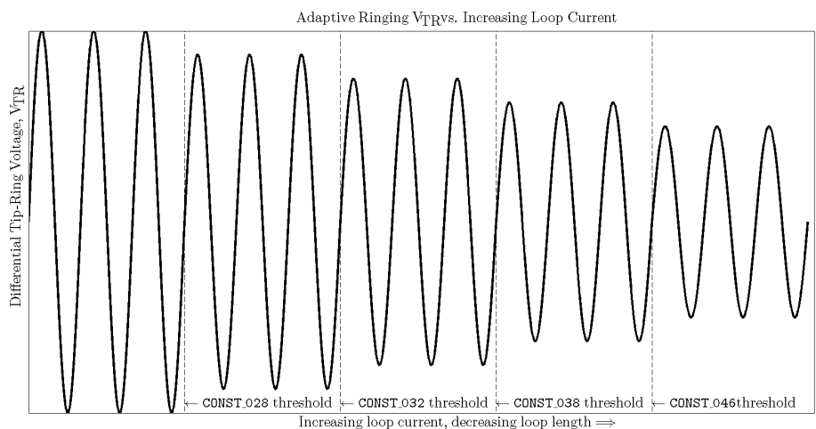
Figure 23. Adaptive Ringing
