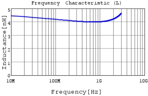
LQP03TN4N0B02 L
