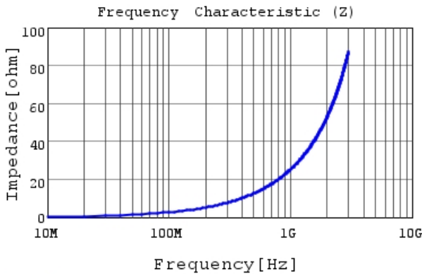
LQP03TN4N0B02 |Z|
