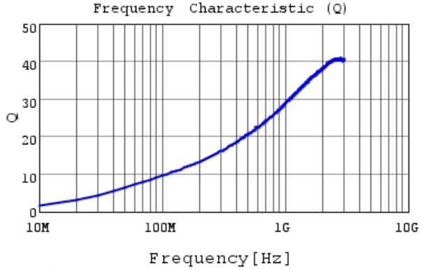
LQP03TN4N0B02 Q
